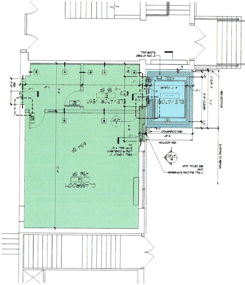
Partial Floor Plan – Proposed Elevator
