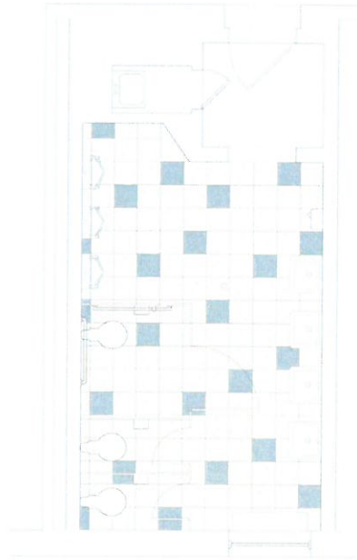
Girl's Toilet Floor Layout
