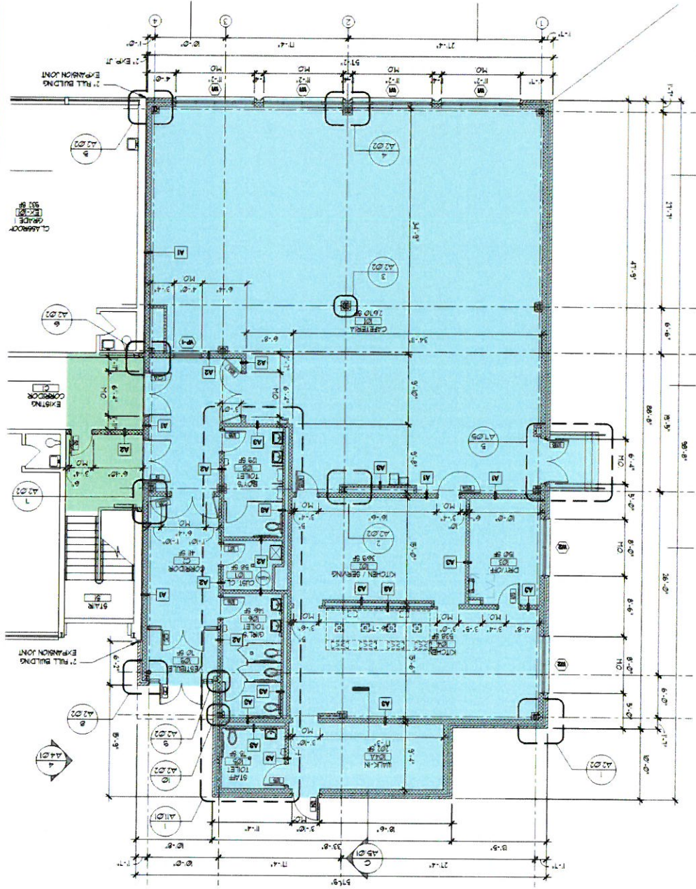
Floor Plan – Proposed Kitchen/ Cafeteria
